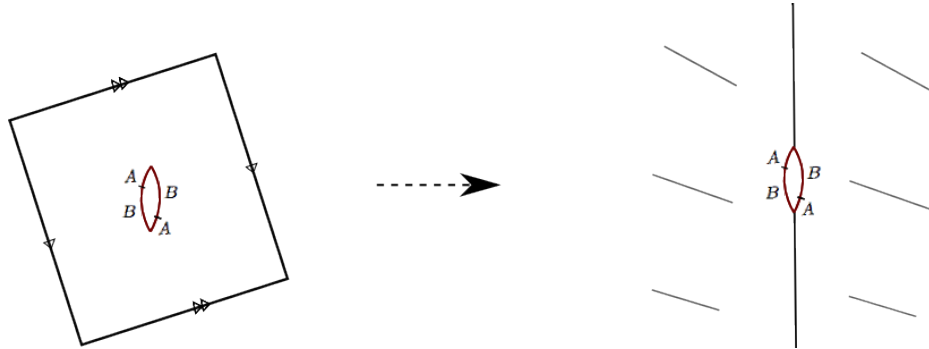
FIGURE 1. ( An example of a half-plane structure. ) The genus-2 surface (on the left) is obtained by an isometric identifications on sub-intervals of a slit of irrational slope on a flat torus. The corresponding Teichmüller ray “stretches” the singular-flat metric in the horizontal direction. A half-plane differential of order 2 on a punctured torus (on the right) then arises as the Gromov-Hausdorff limit when basepoints are taken to lie on the critical graph.
