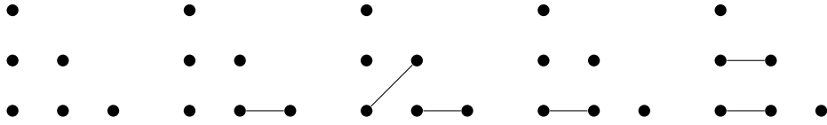
Figure 3: The set of gravity diagrams GD_{(Zig_6)_5}(3, -1, -1, -1, 0) .
