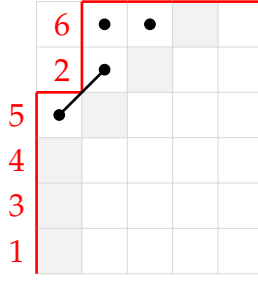
Figure 4: A unified diagram U = (\mathbf{s}, \sigma, \varphi, D) for G = \text{Car}_6 with \mathbf{a} = (1, \dots, 1) (net flow labels suppressed) and shifted out-degree vector \mathbf{t} = (3, 1, 1, 1, 0) . The \mathbf{t} -Dyck path is \mathbf{s} = (4, 2, 0, 0, 0) with parking label \sigma = 134526 , and D is a gravity diagram in \text{GD}_{G|_5}(1, 1, -1, -1) = \text{GD}_{G|_5}(\alpha_1 + 2\alpha_2 + \alpha_3) .
