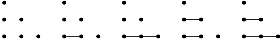
Figure 2: The set of gravity diagrams GD_{(Car_6)_5}(3, -1, -1, -1, 0) .
