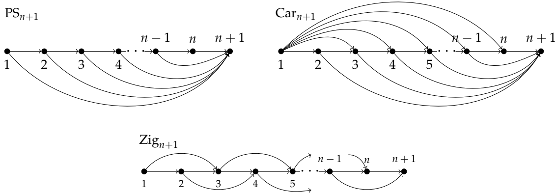
Figure 1: The Pitman-Stanley, caracol, and zigzag graphs.
