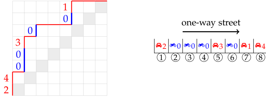
Figure 5: The multi-labeled Dyck path ((2, 3, 1, 0, 0, 2, 0, 0), 24003001) \in M(8, 4) corresponds to the parking preference pair \mathbf{p} = \{2, 2, 3, 6\} \times (6, 1, 2, 1) ; the final parking arrangement is given on the right.
